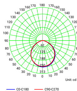
Luminous Intensity Distribution Curve - 3018.107.1TL
