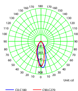
Luminous Intensity Distribution Curve - 3015.105.8TL
