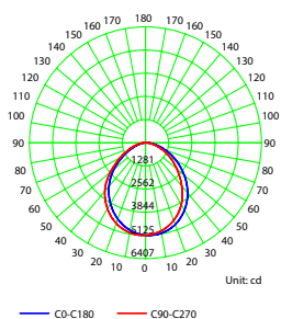
Luminous Intensity Distribution Curve - 5512.125.10L
