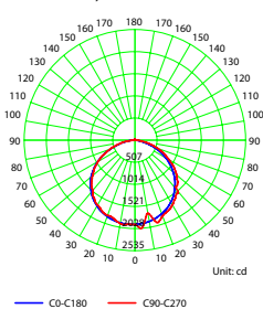
Luminous Intensity Distribution Curve - 4069.147.4TL
