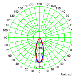
Luminous Intensity Distribution Curve - 6041.110.8XL
