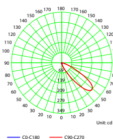
Luminous Intensity Distribution Curve - 2528.003.2TL
