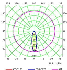
Luminous Intensity Distribution Curve - 6024.112.8PL
