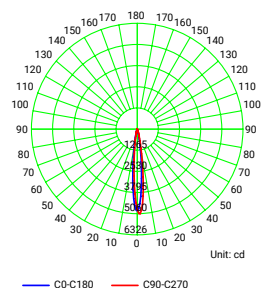
Luminous Intensity Distribution Curve - 3063.302.8TL
