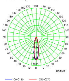
Luminous Intensity Distribution Curve - 2508.111.7TL
