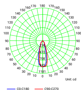
Luminous Intensity Distribution Curve - 1524.301.xXL
