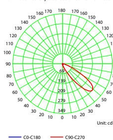
Luminous Intensity Distribution Curve - 2527.003.2TL
