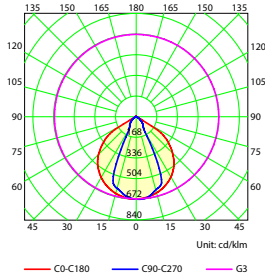
Luminous Intensity Distribution Curve - 2041.103.xPL
