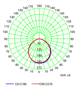
Luminous Intensity Distribution Curve - 2060.107.1TL
